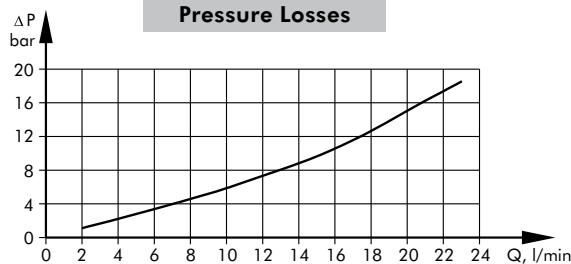
Pressure Losses
